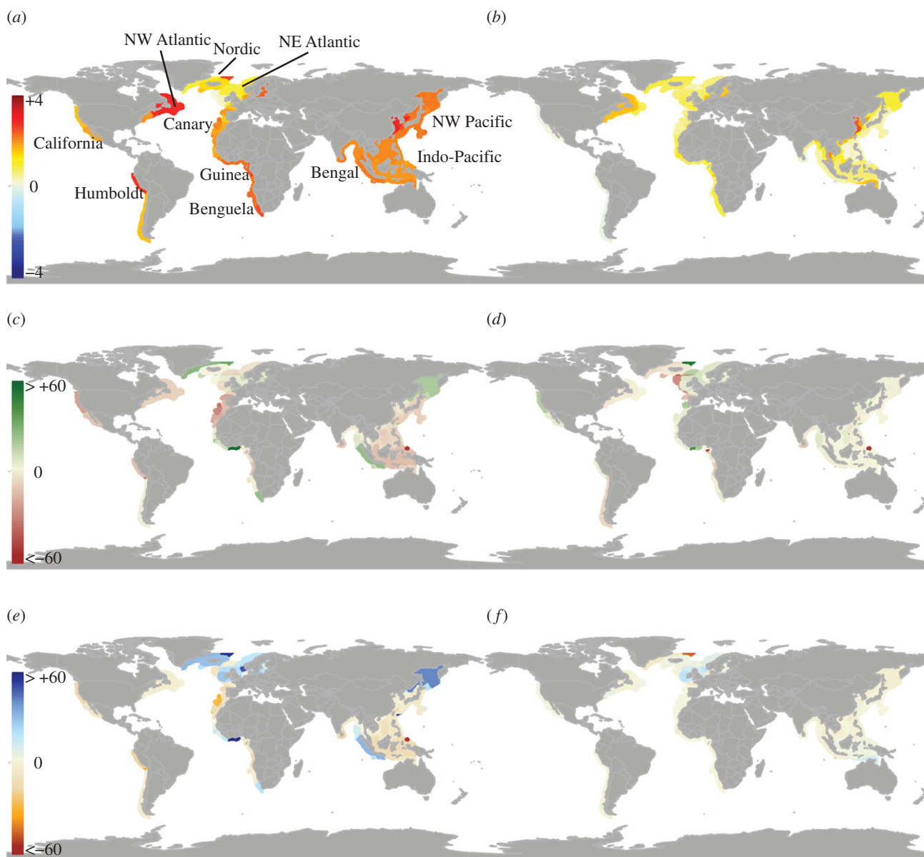
Figure 1. Mean-predicted relative changes for 2050 under the SREASA1B scenario. Maps of change in (a) mixed-layer depth temperature; (b) near sea floor temperature ( ^{\circ}\text{C} ); and percentage changes in: (c) density of phytoplankton and (d) biomass density of detritus; (e) biomass density of pelagic predators and (f) biomass density of benthic detritivores.
